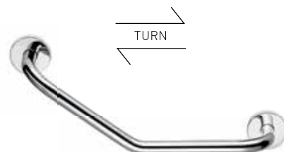
0400-A03 Grab-Bar Λαβή W42 x D10,5 x H16,5 (cm) CHROME COLORS FINISHES
